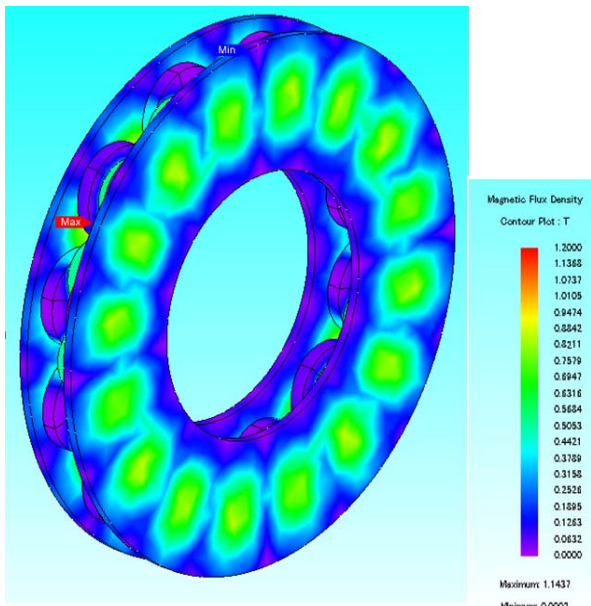
Fig. 1. Rotor-PM flux density distribution in the small double-sided inner-rotor AFPM synchronous wind-generator.
